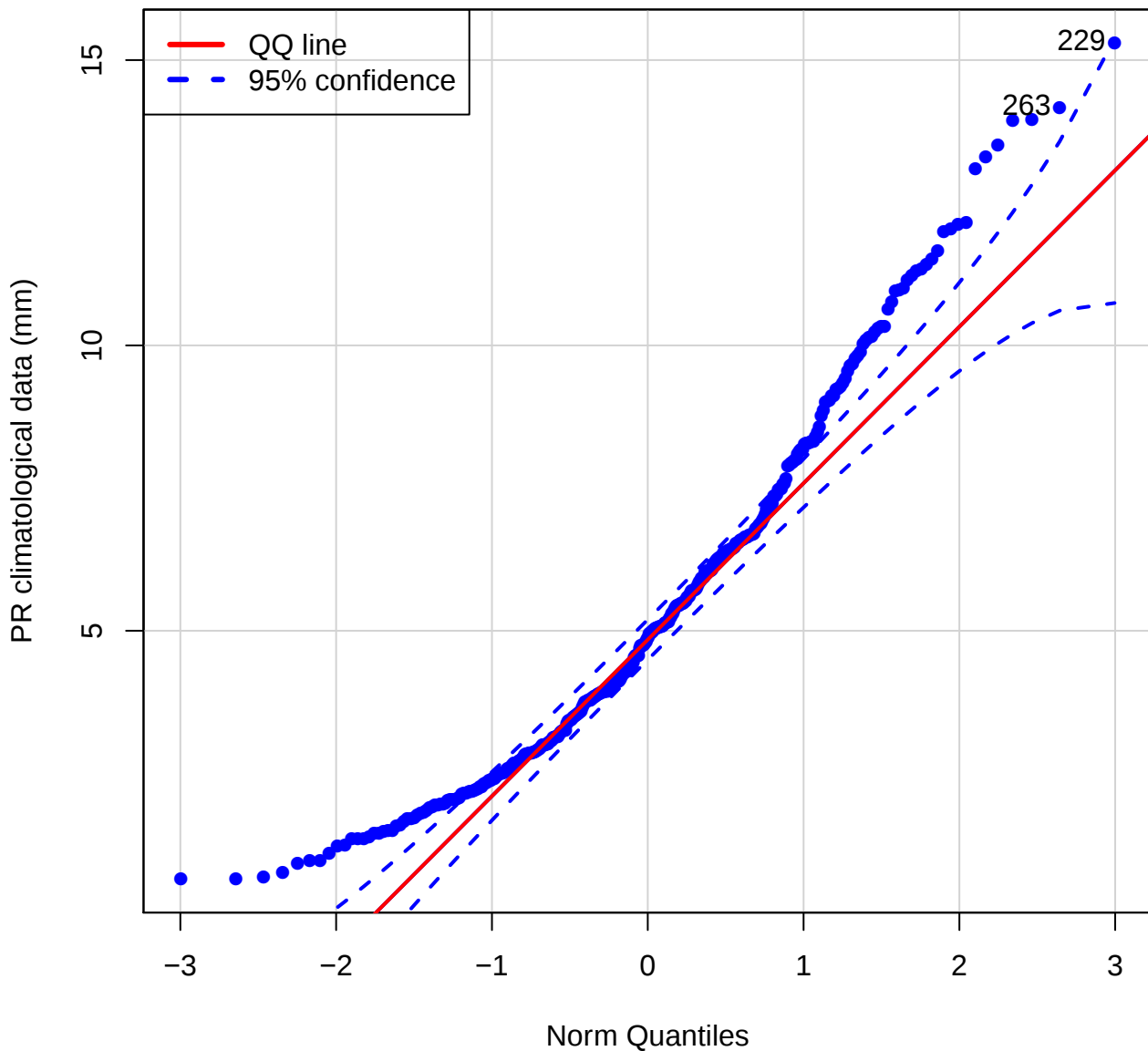
QQ plot (Pr of FDFD)
