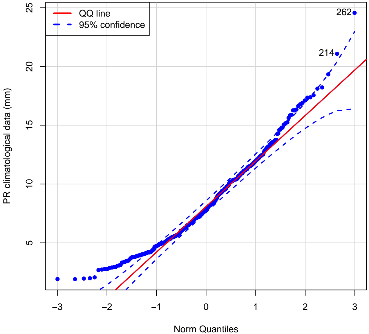
QQ plot (Pr of FDFL)
