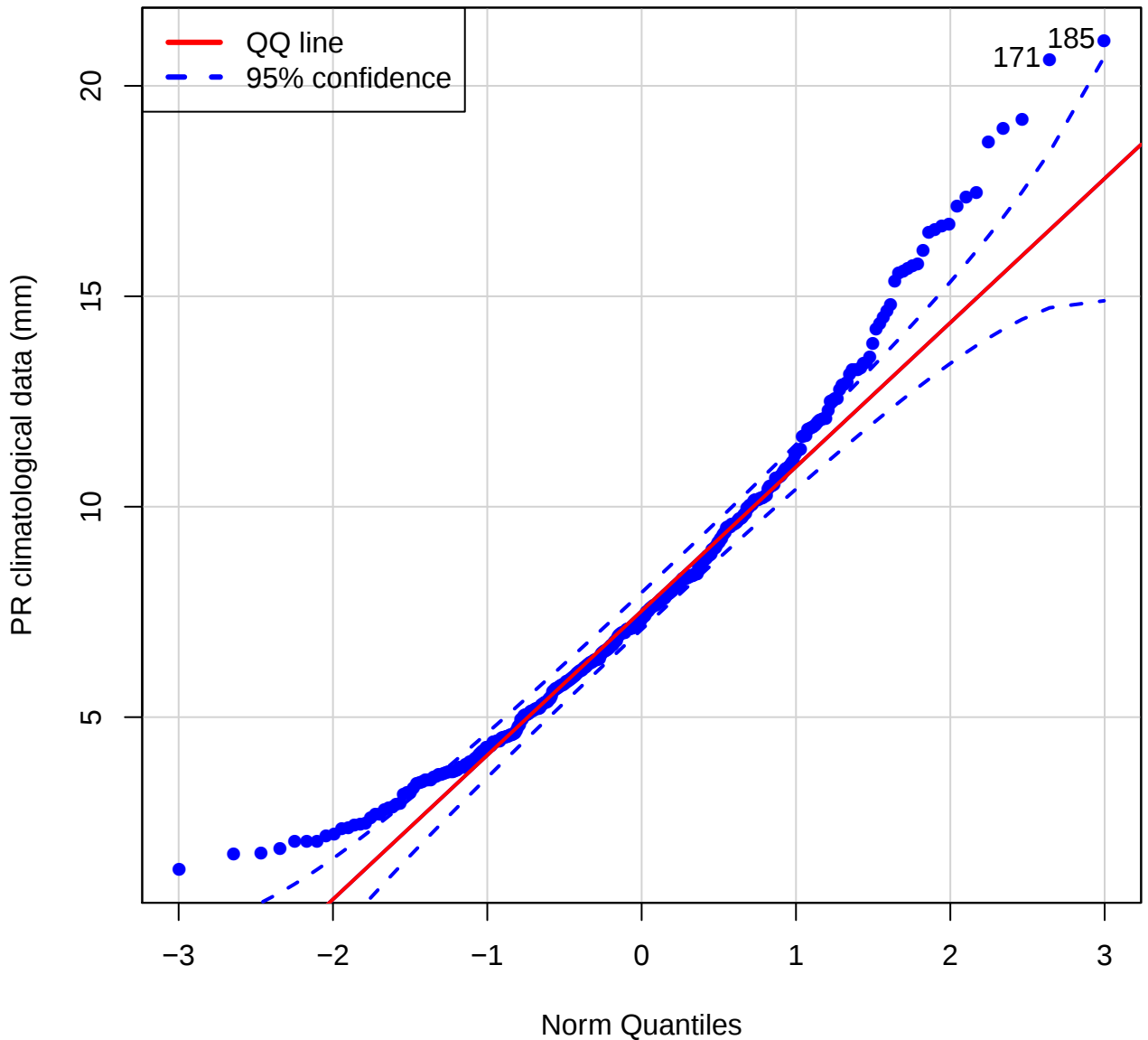
QQ plot (Pr of FSDC)
