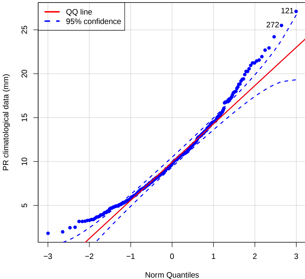
QQ plot (Pr of GMRN)
