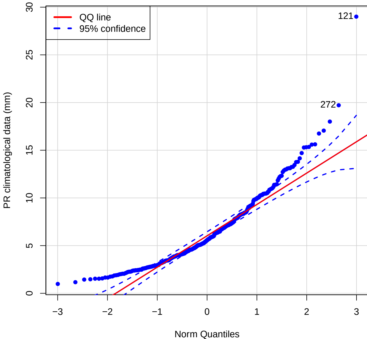
QQ plot (Pr of LAMQ)
