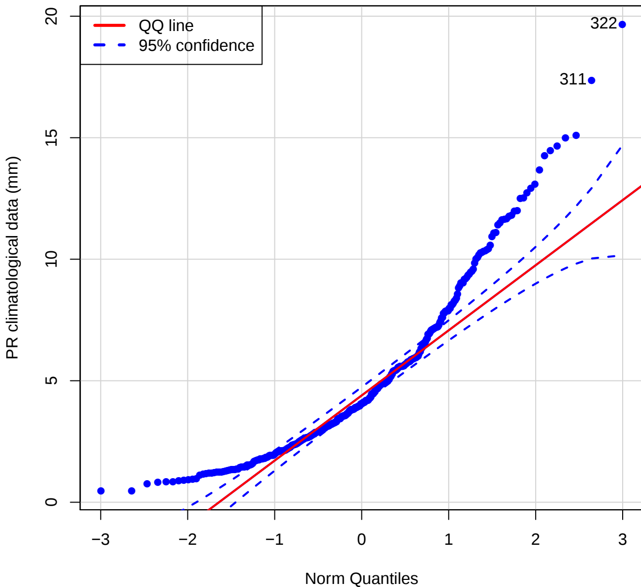
QQ plot (Pr of LFRC)
