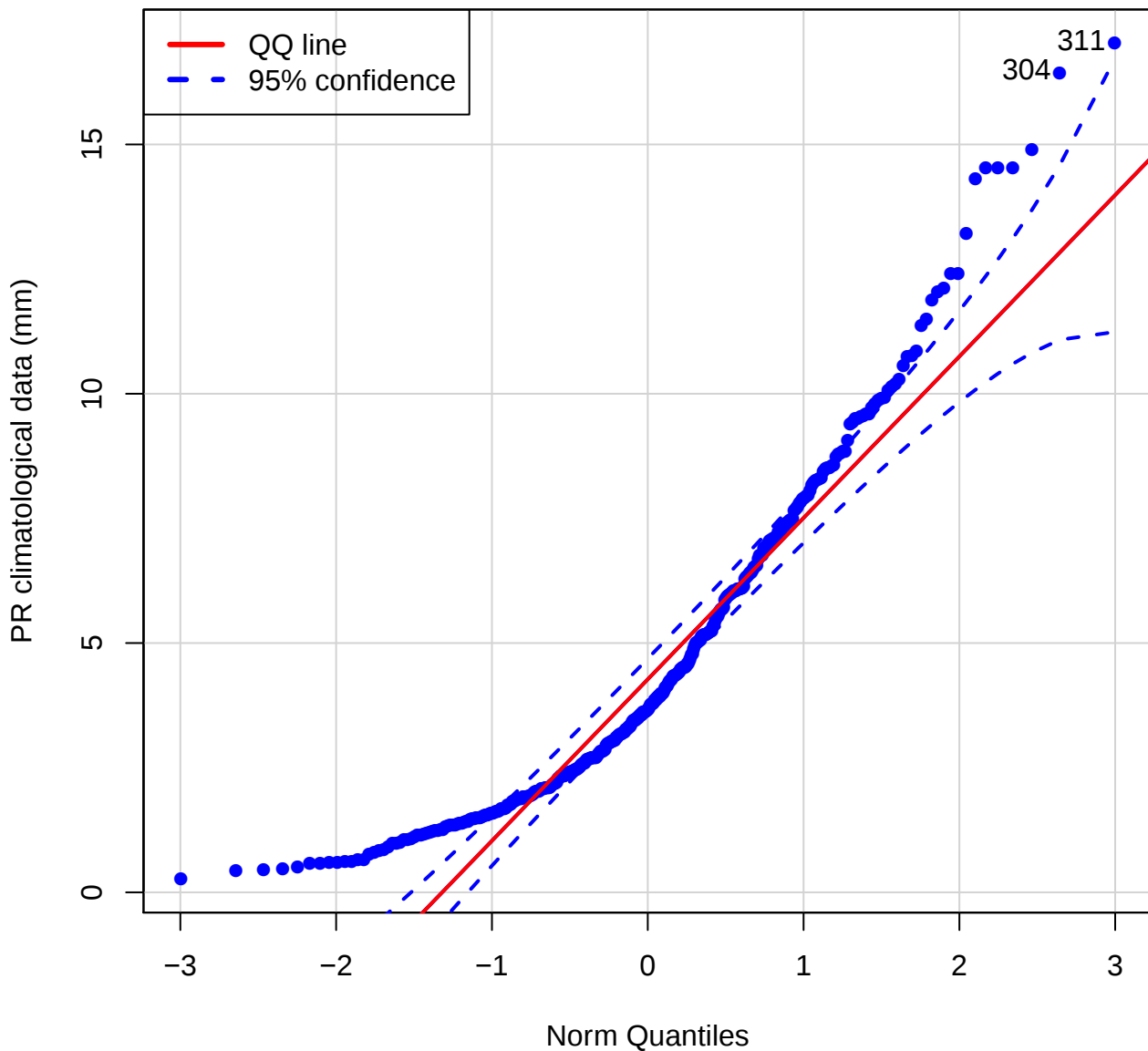
QQ plot (Pr of LFRS)
