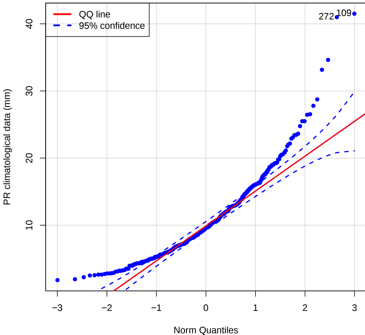
QQ plot (Pr of LORR)
