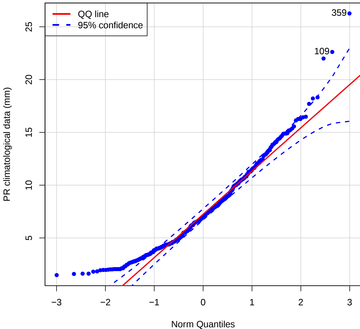
QQ plot (Pr of MACB)
