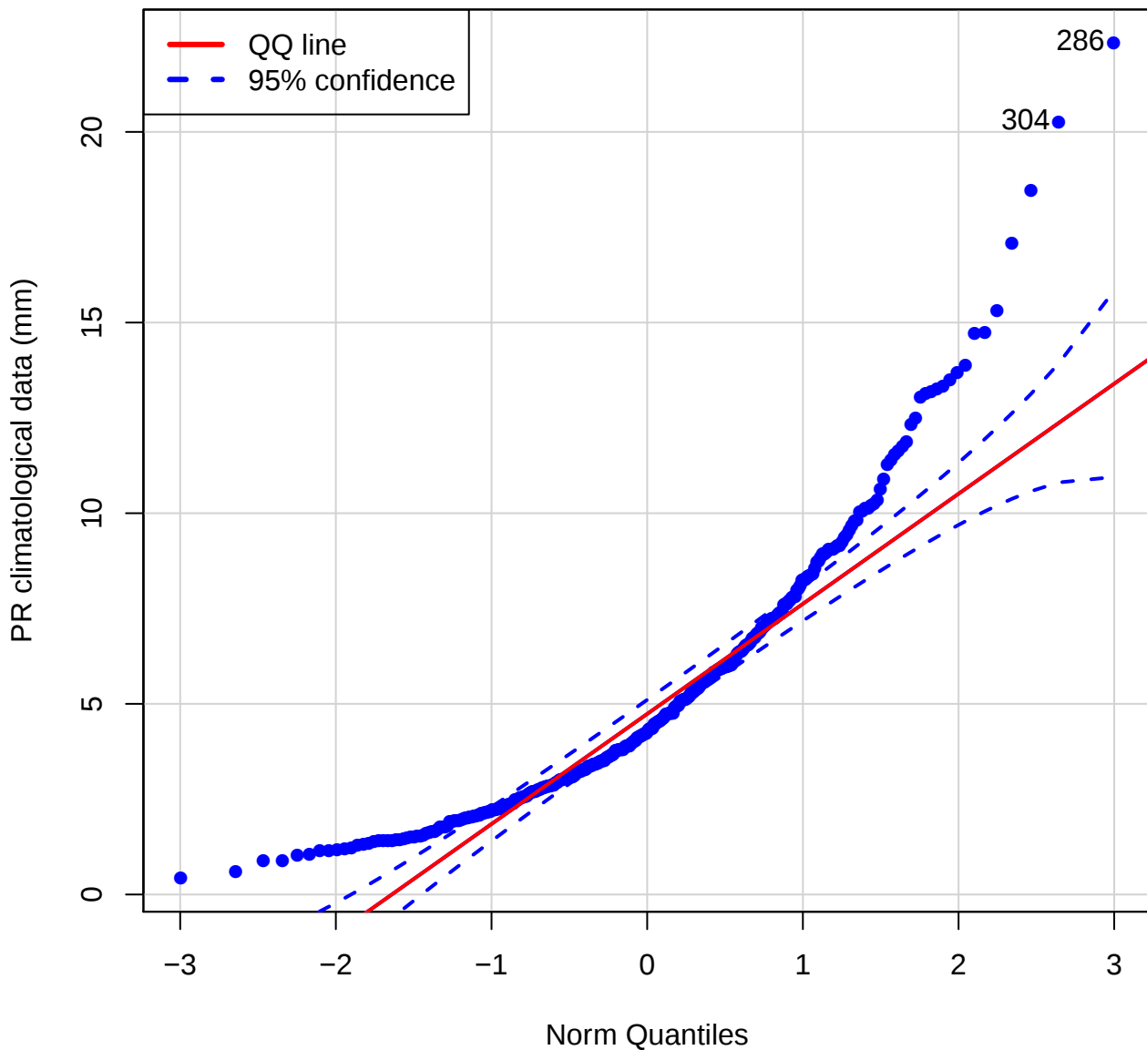
QQ plot (Pr of MARN)
