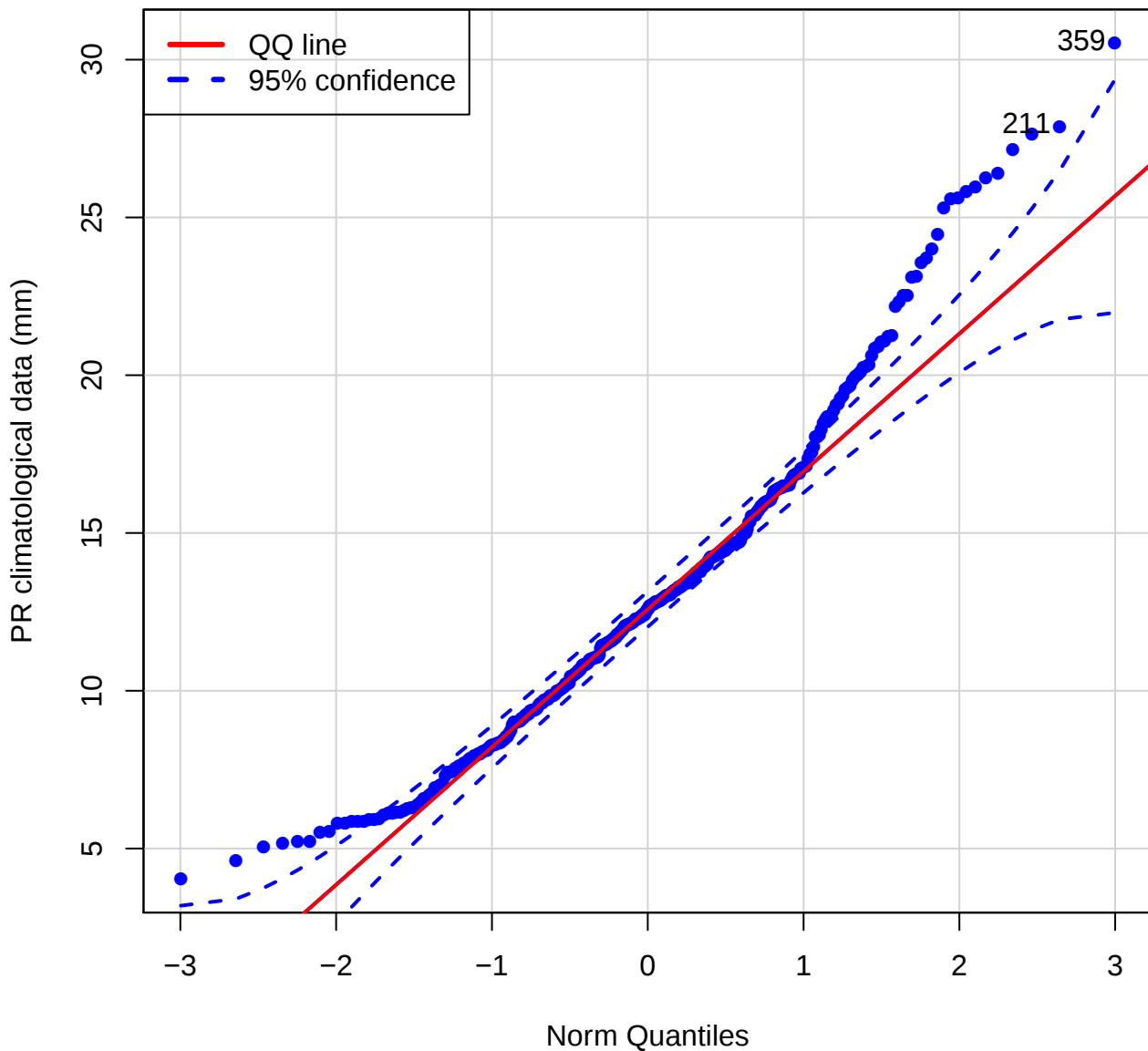
QQ plot (Pr of MRRC)
