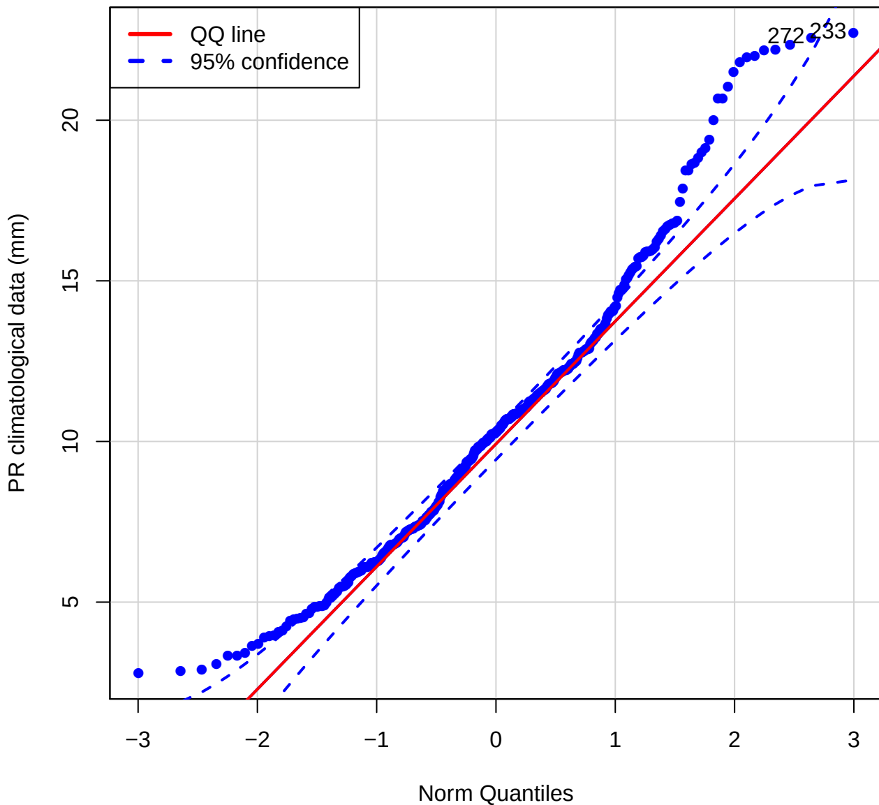
QQ plot (Pr of MRRD)
