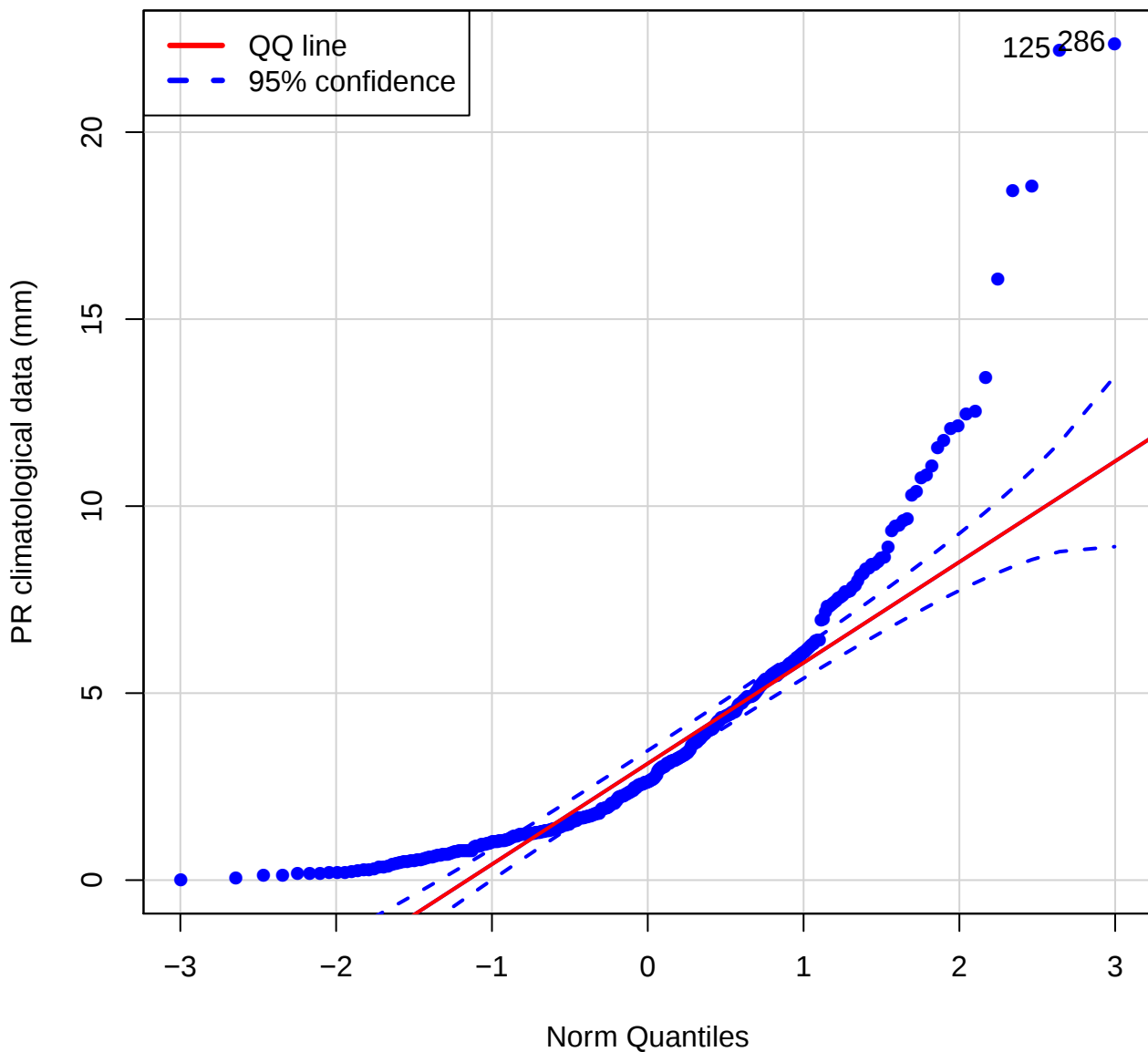
QQ plot (Pr of PANS)
