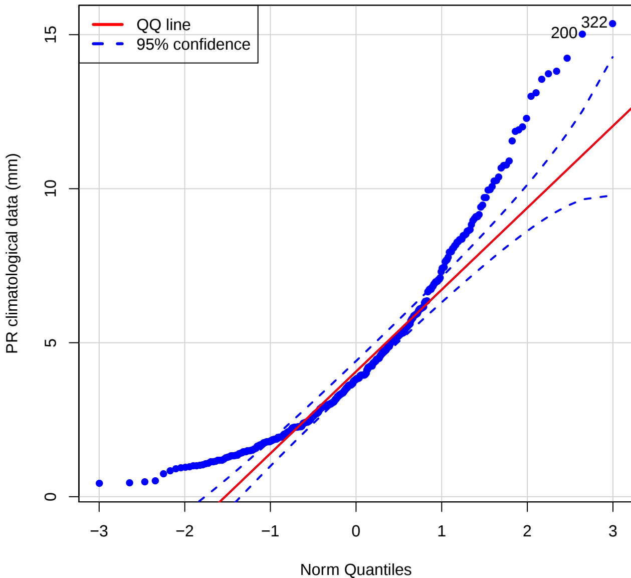
QQ plot (Pr of ROBP)
