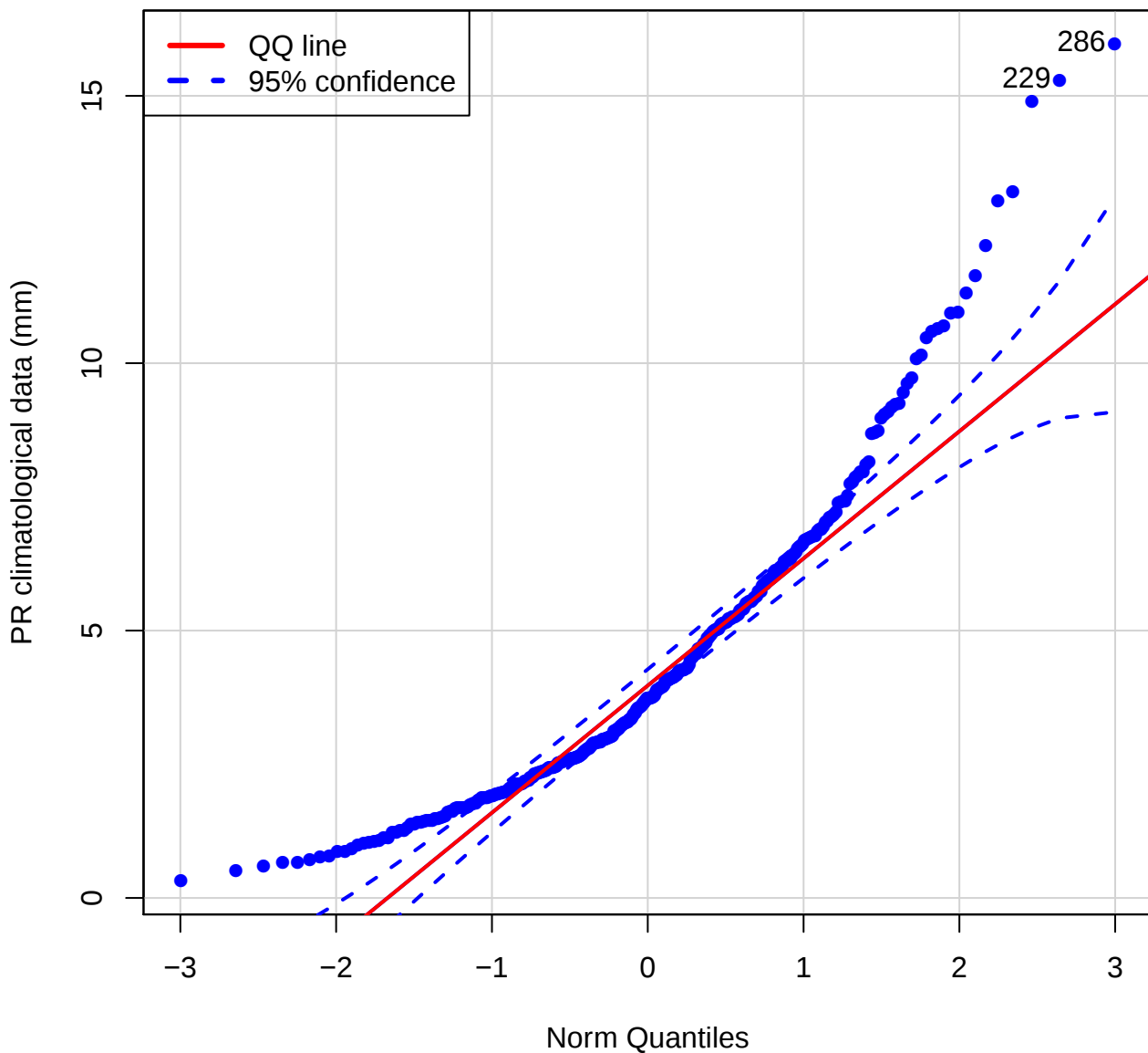
QQ plot (Pr of STAN)
