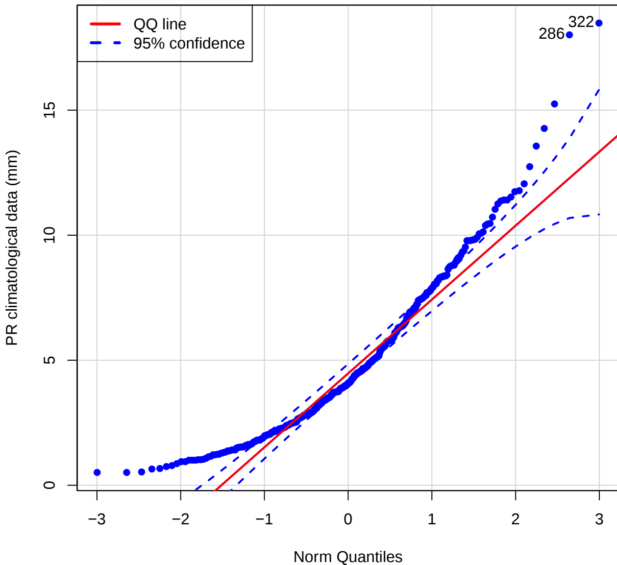
QQ plot (Pr of STEB)
