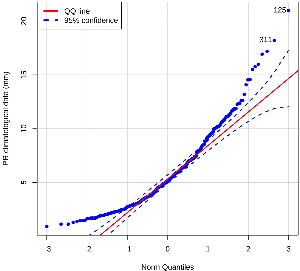
QQ plot (Pr of STEG)
