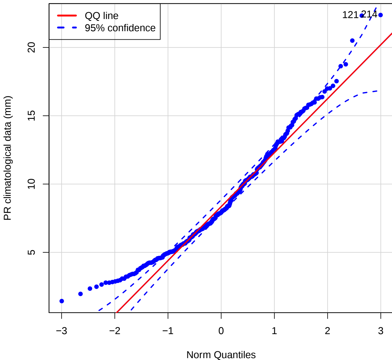
QQ plot (Pr of STJB)
