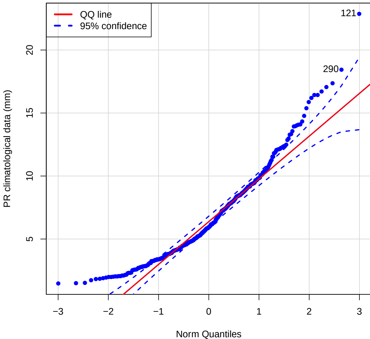
QQ plot (Pr of STJL)
