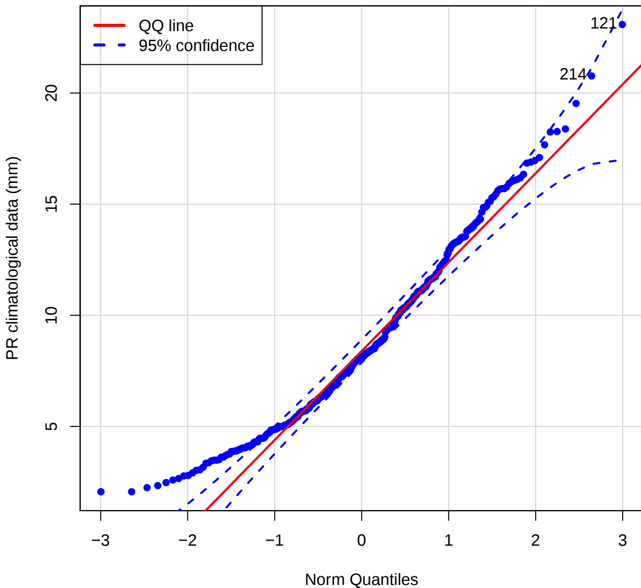
QQ plot (Pr of STJR)
