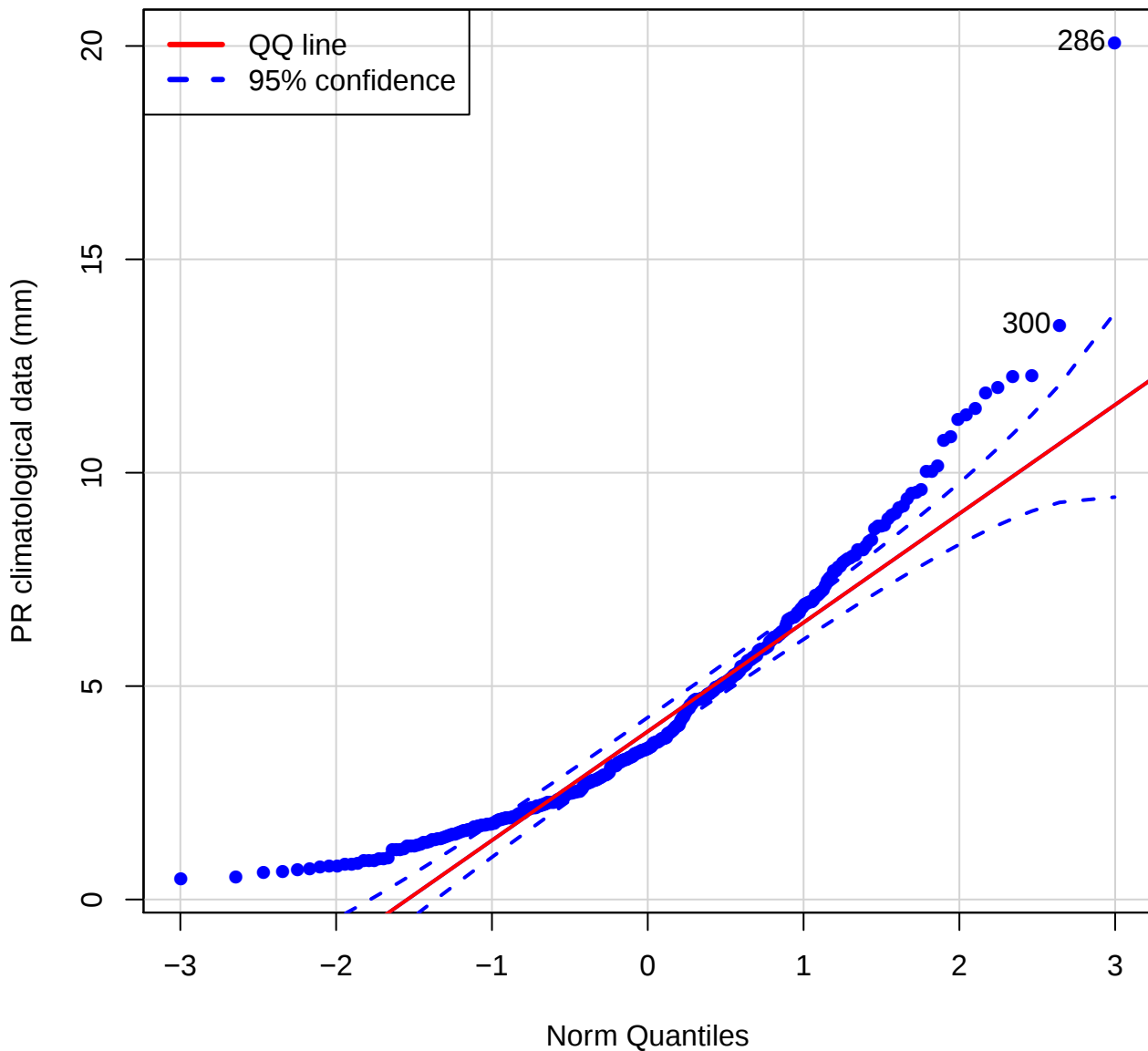
QQ plot (Pr of STLC)
