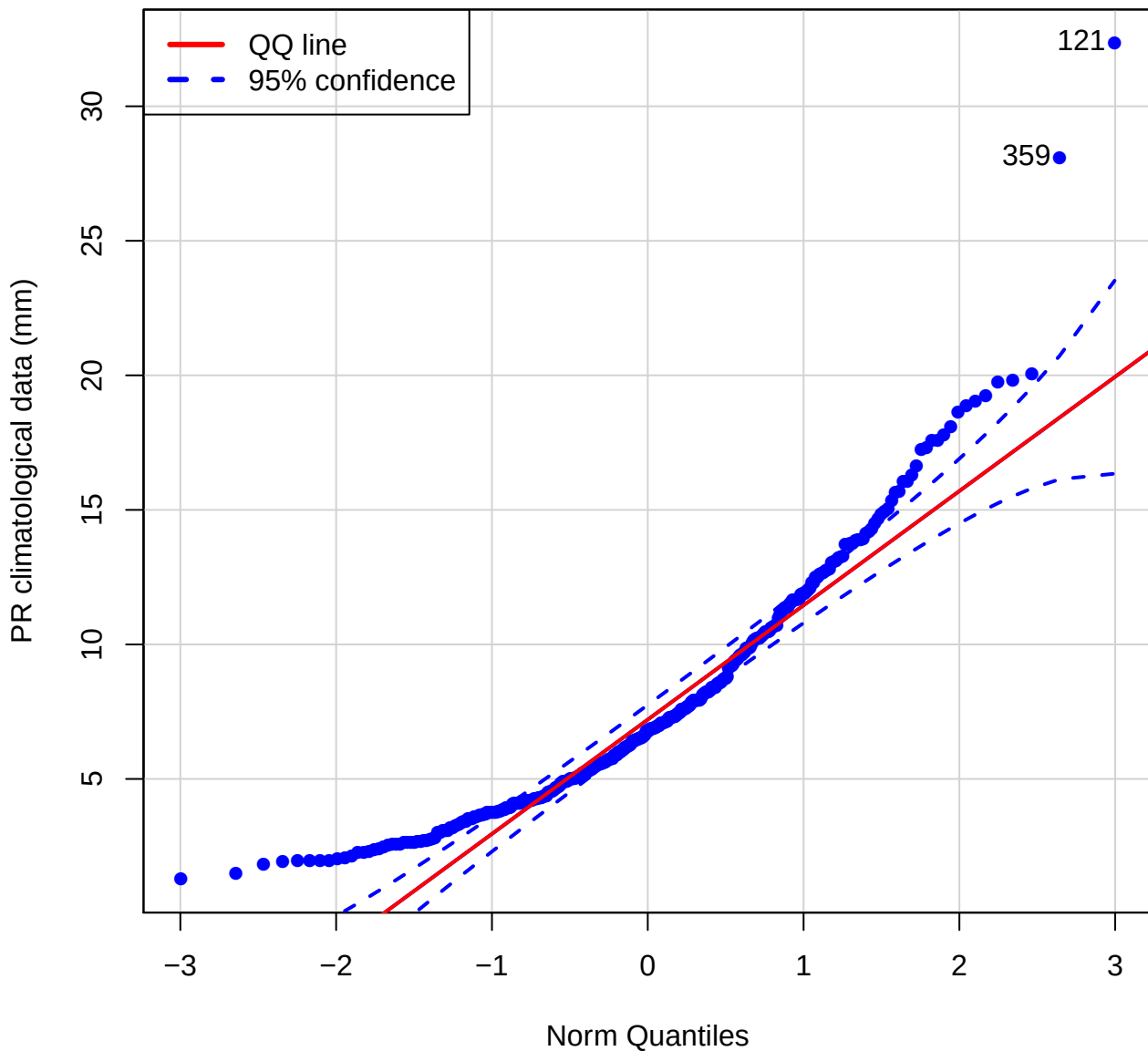
QQ plot (Pr of STMB)
