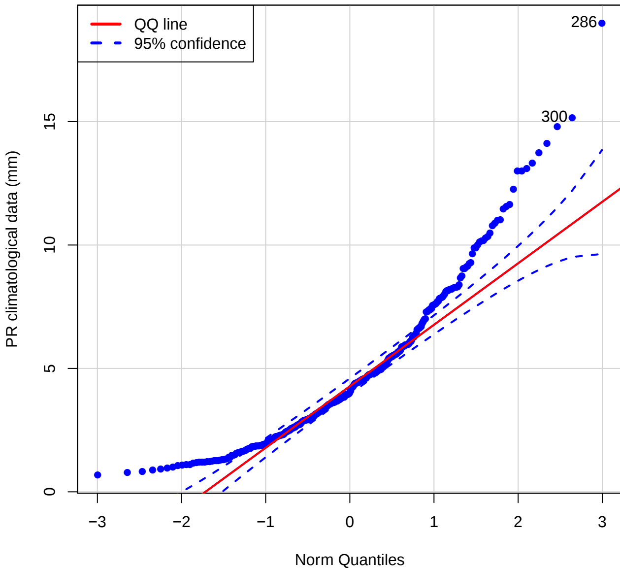
QQ plot (Pr of TILG)
