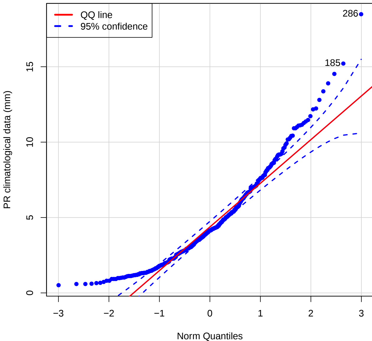
QQ plot (Pr of TILP)
