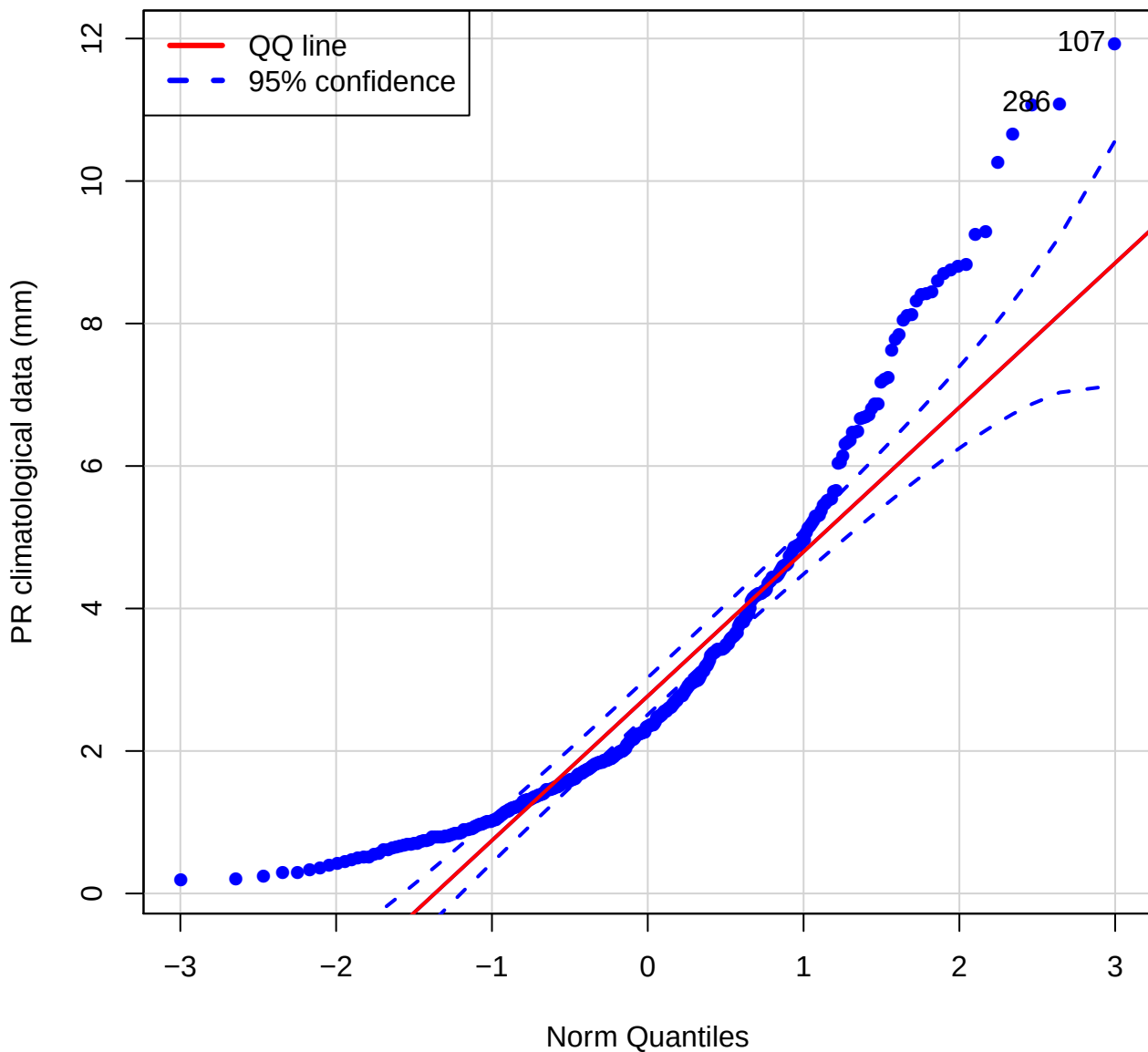
QQ plot (Pr of TRTC)
