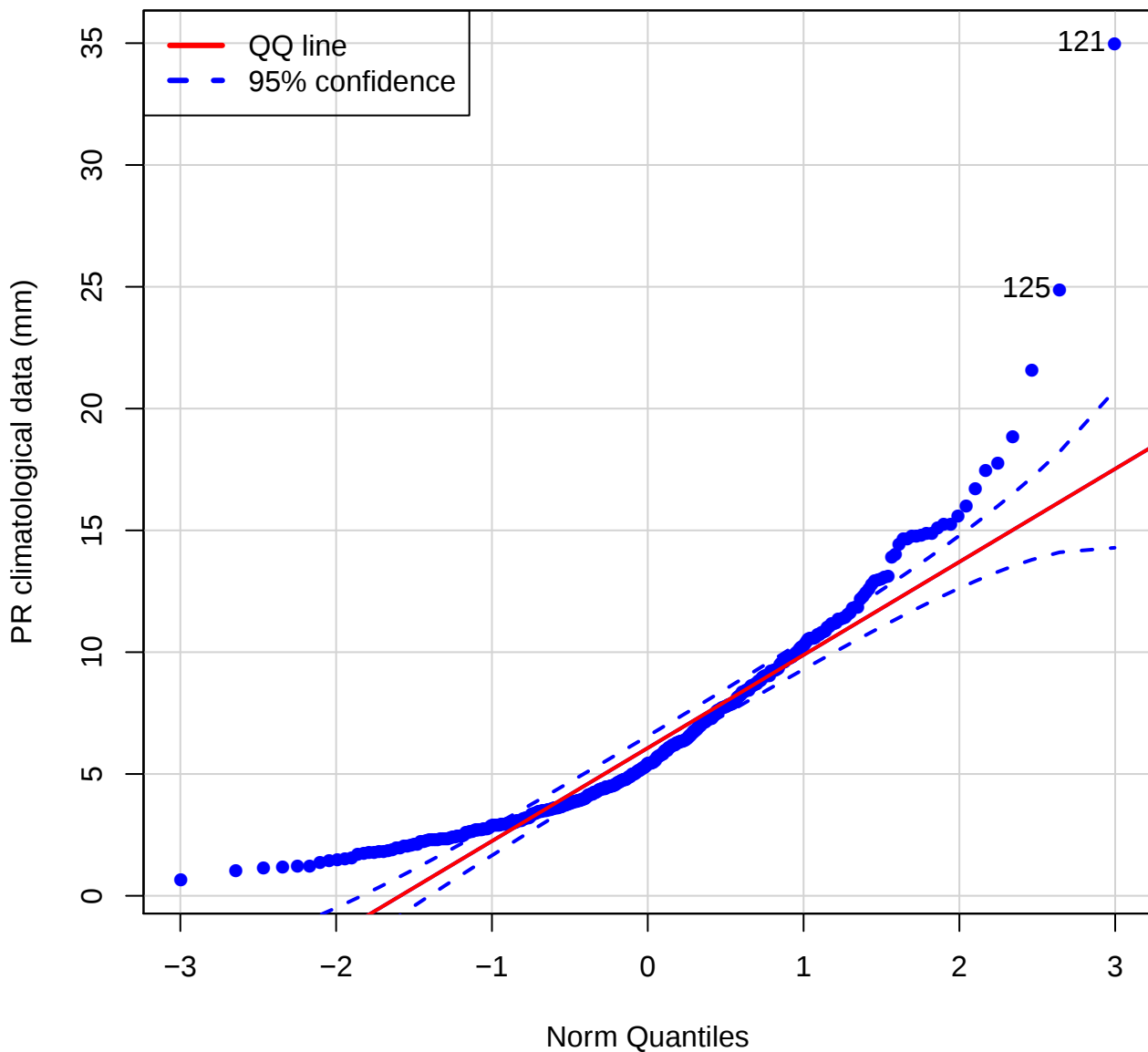
QQ plot (Pr of TRTR)
