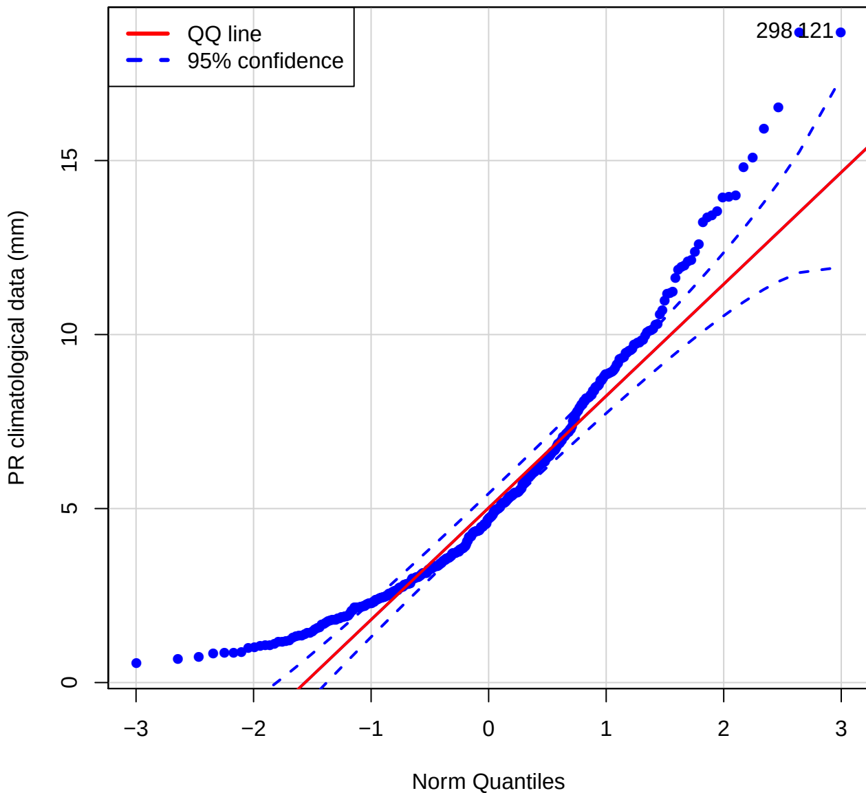
QQ plot (Pr of TRTS)
