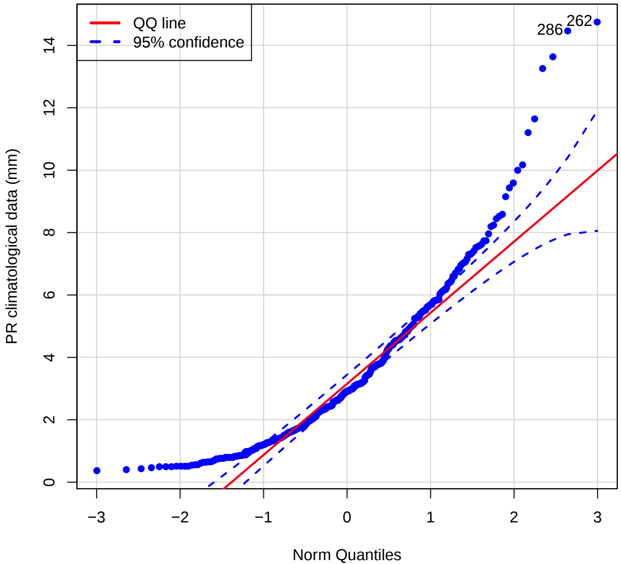
QQ plot (Pr of VCLC)
