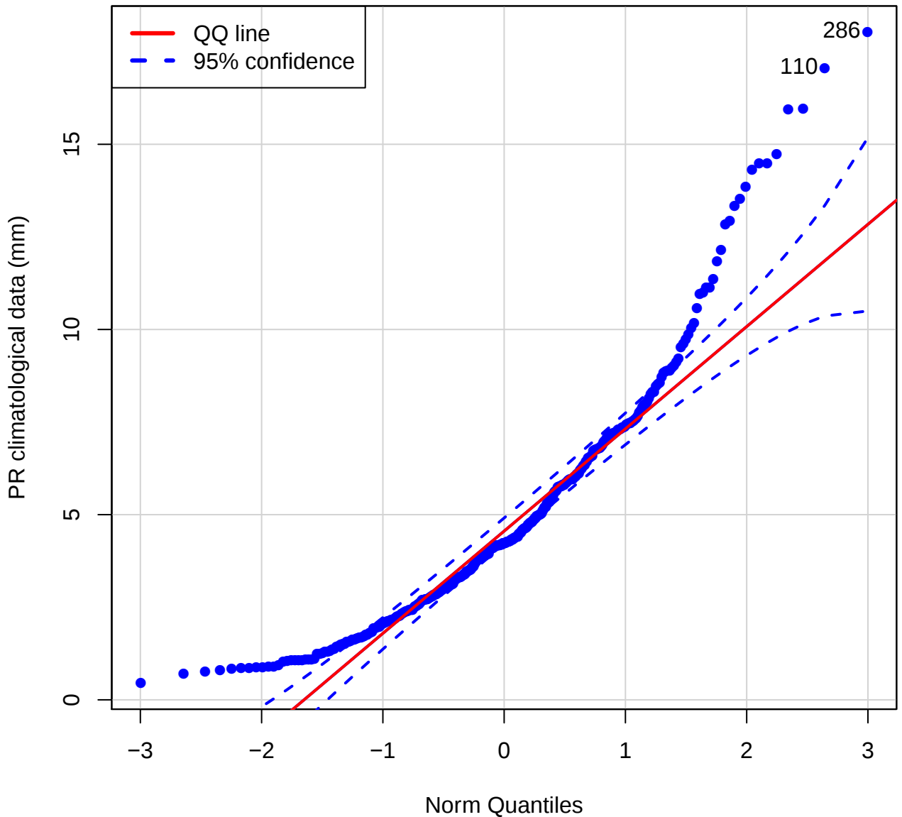
QQ plot (Pr of VCLR)
