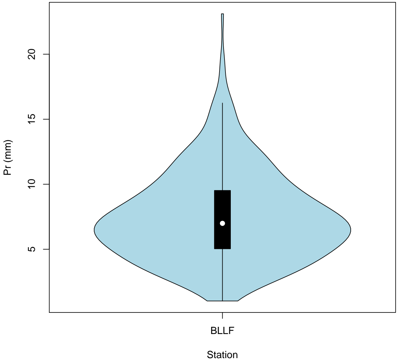
Violin Plots of Pr (BLLF)
