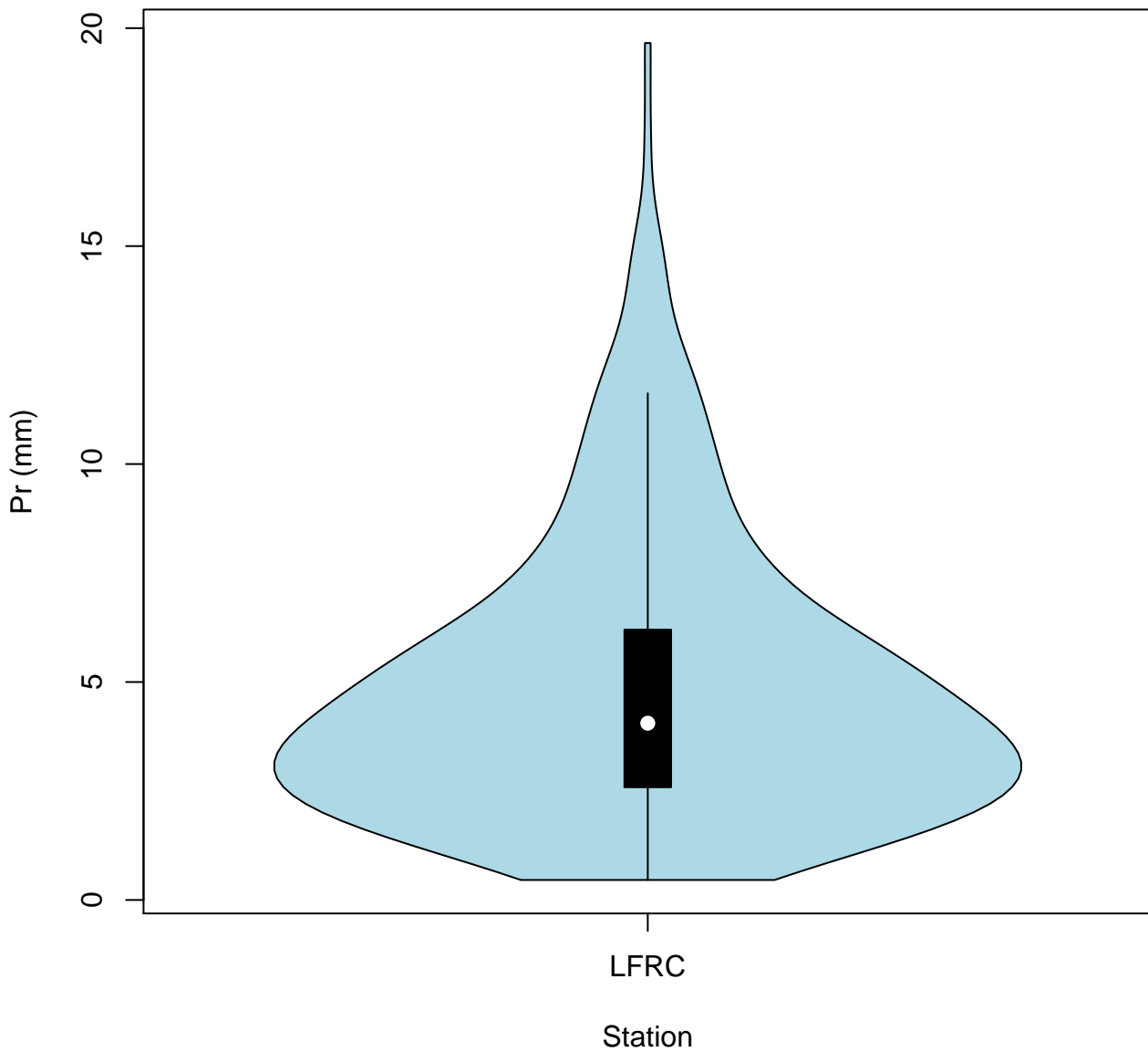
Violin Plots of Pr (LFRC)
