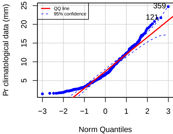
QQ plot (BASP)
