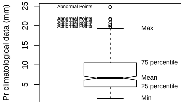
Box plot (BASP)
