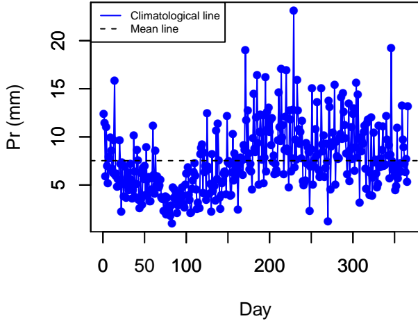
Climatology (BLLF)
