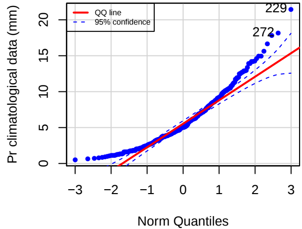
QQ plot (CARB)
