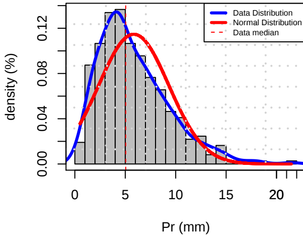
Histogram Distribution (CARB)
