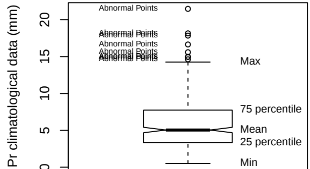
Box plot (CARB)
