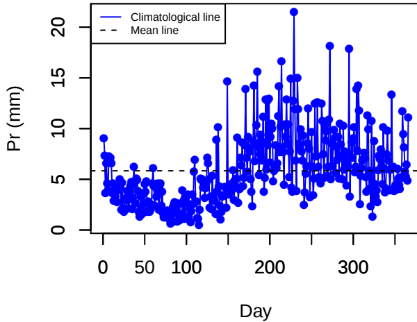
Climatology (CARB)
