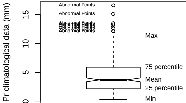
Box plot (DIAM)
