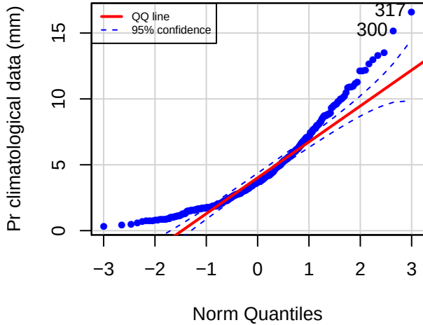
QQ plot (DIAM)
