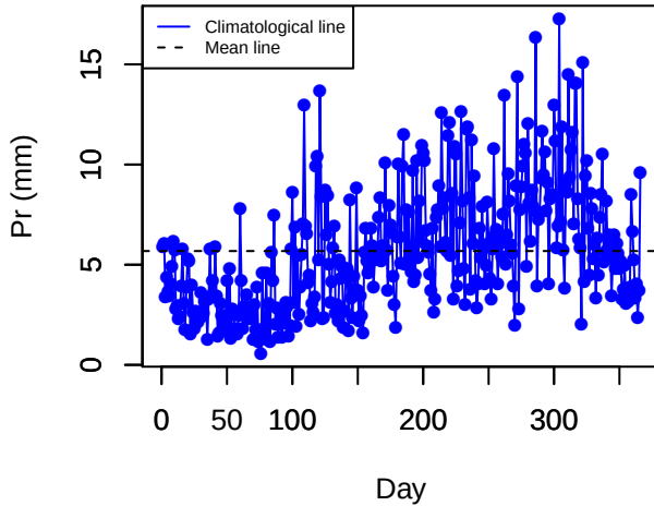
Climatology (DUCO)
