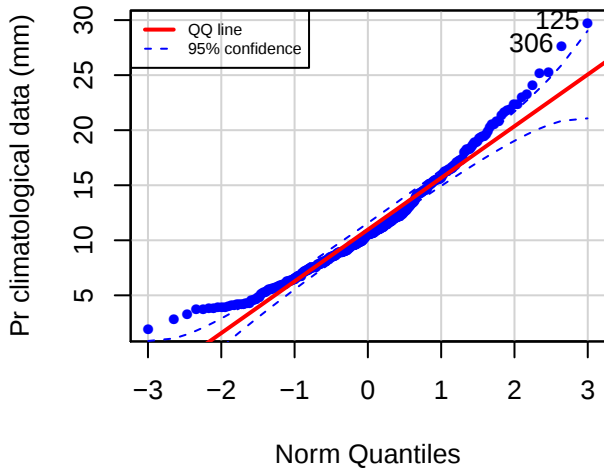
QQ plot (FDFC)
