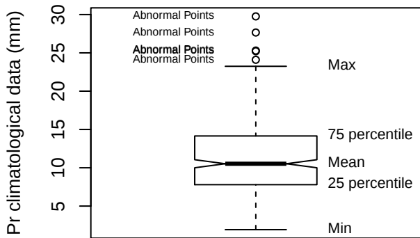
Box plot (FDFC)
