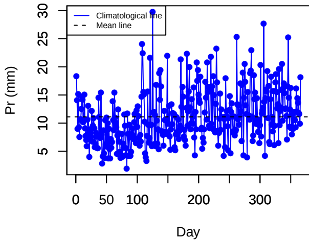
Climatology (FDFC)
