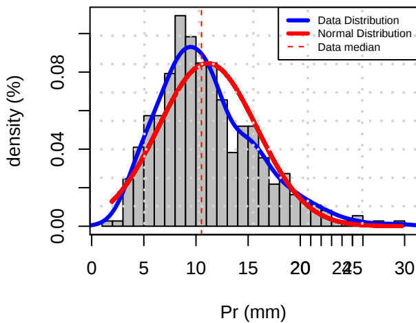
Histogram Distribution (FDFC)
