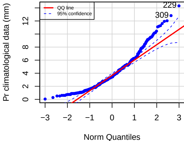
QQ plot (FDFF)
