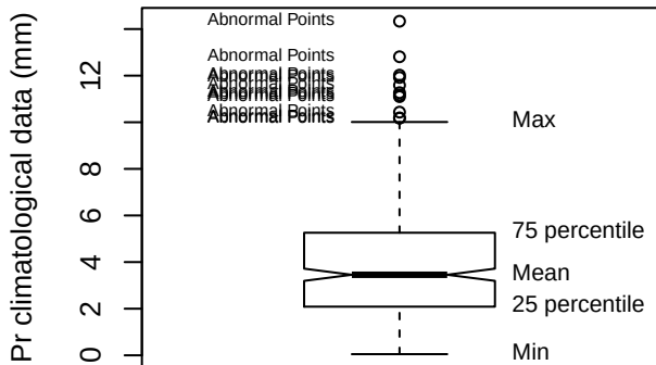
Box plot (FDFF)
