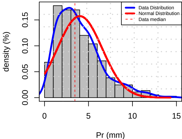
Histogram Distribution (FDFF)
