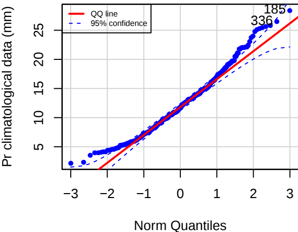
QQ plot (FSDG)
