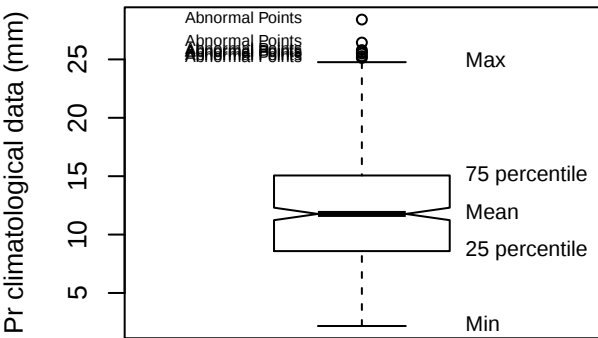
Box plot (FSDG)
