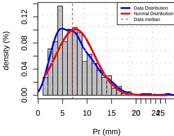
Histogram Distribution (MACB)
