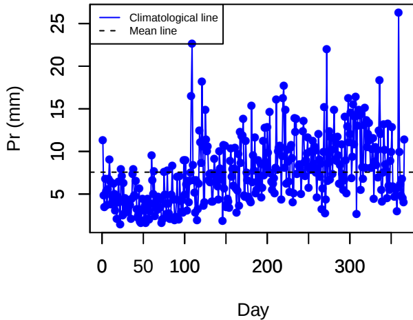
Climatology (MACB)
