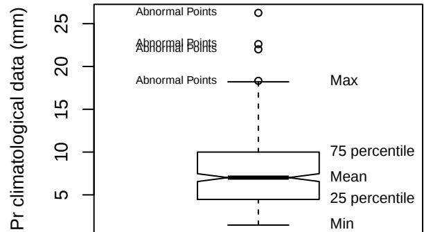
Box plot (MACB)
