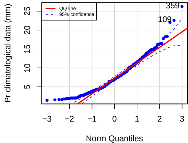
QQ plot (MACB)
