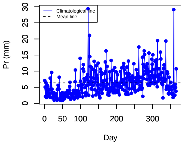
Climatology (MARB)
