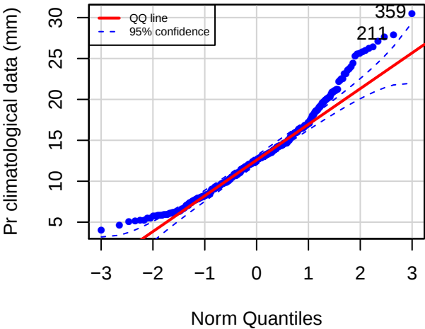
QQ plot (MRRC)
