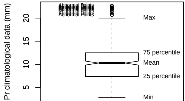
Box plot (MRRD)
