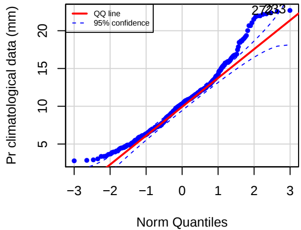
QQ plot (MRRD)
