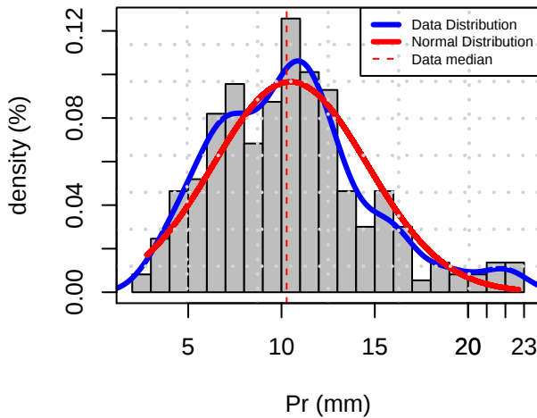
Histogram Distribution (MRRD)
