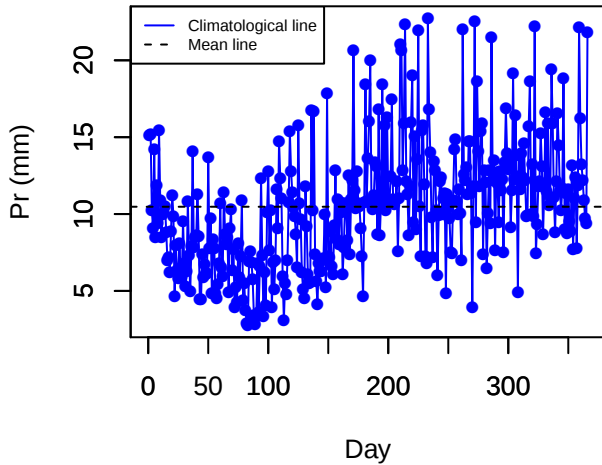
Climatology (MRRD)
