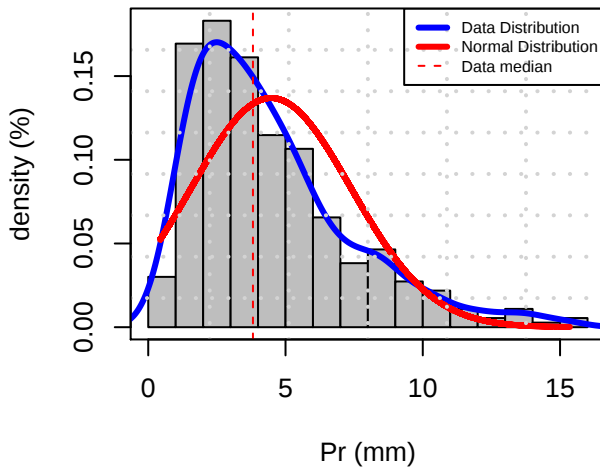
Histogram Distribution (ROBP)
