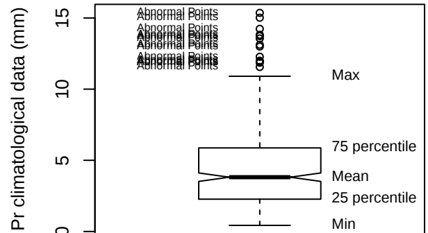
Box plot (ROBP)
