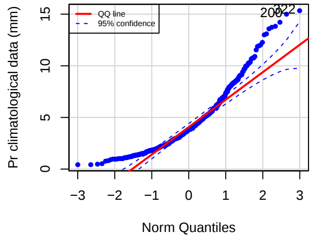
QQ plot (ROBP)
