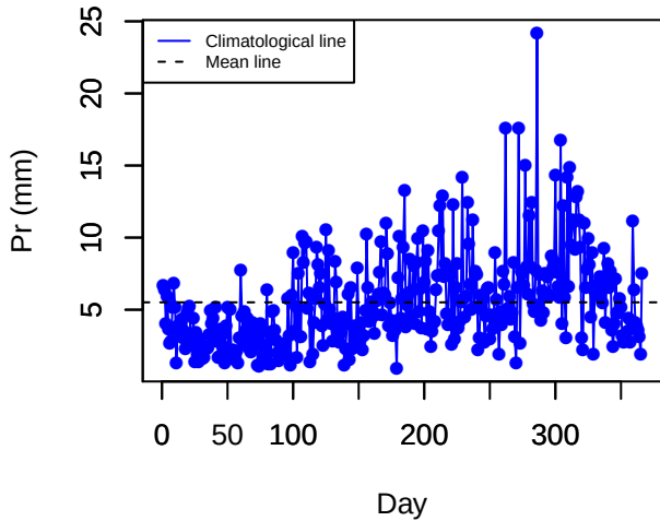
Climatology (RVPE)
