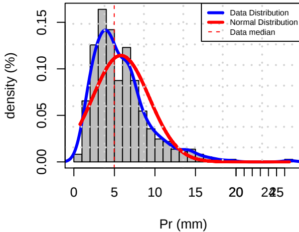
Histogram Distribution (RVPM)
