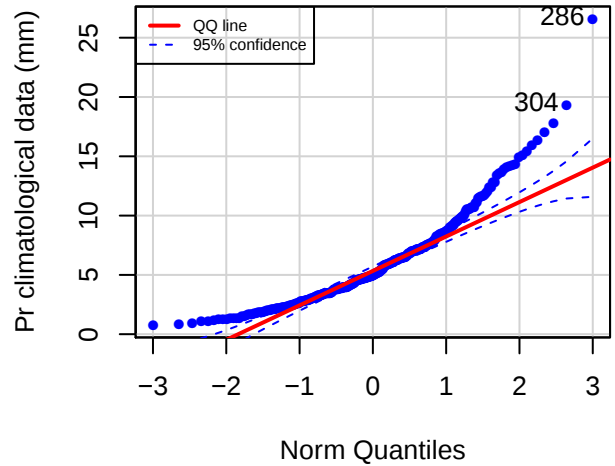
QQ plot (RVPM)
