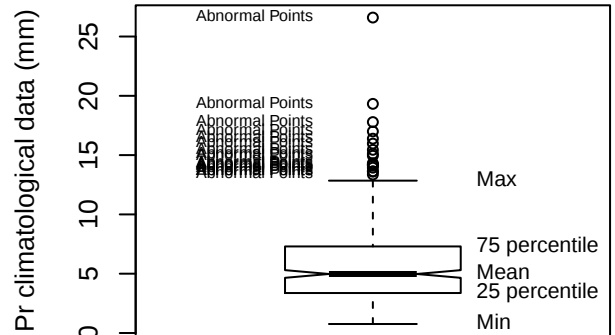
Box plot (RVPM)
