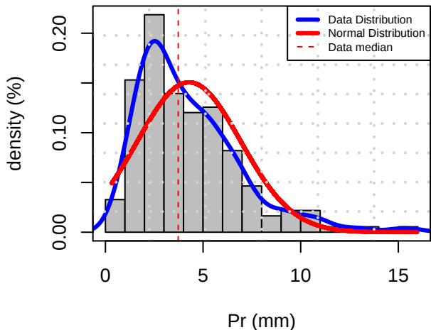
Histogram Distribution (STAN)
