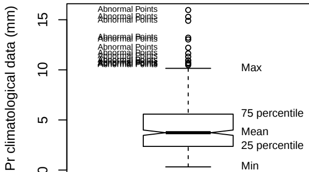
Box plot (STAN)
