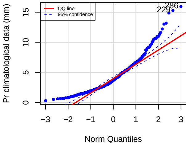
QQ plot (STAN)
