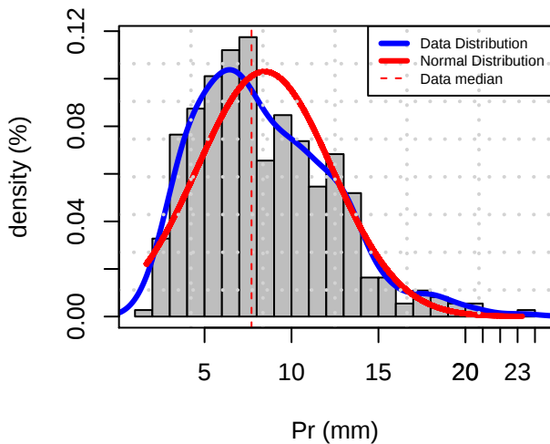
Histogram Distribution (STJO)
