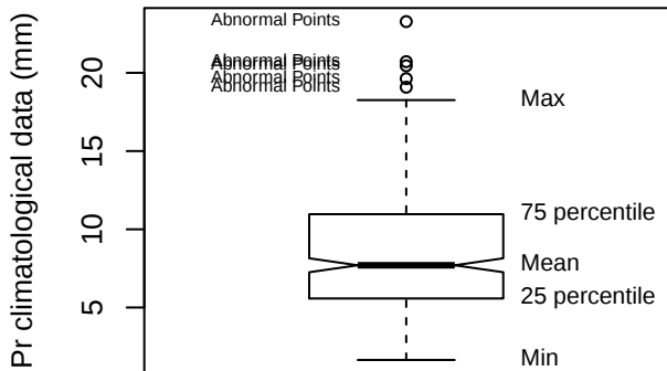
Box plot (STJO)
