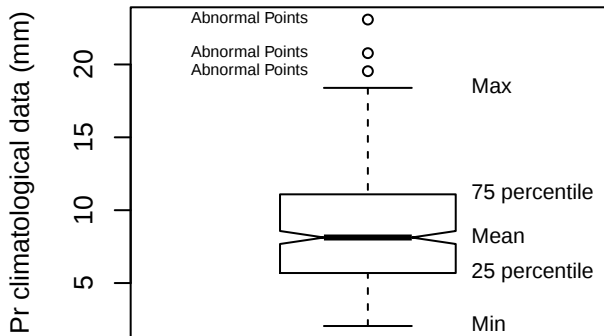
Box plot (STJR)
