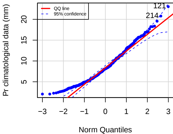
QQ plot (STJR)
