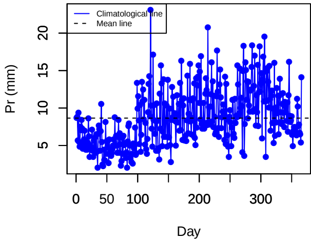
Climatology (STJR)
