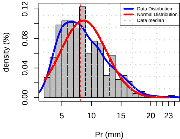
Histogram Distribution (STJR)
