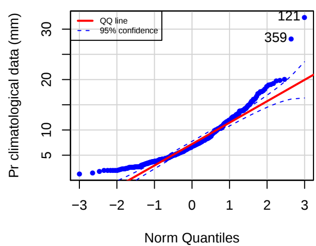
QQ plot (STMB)
