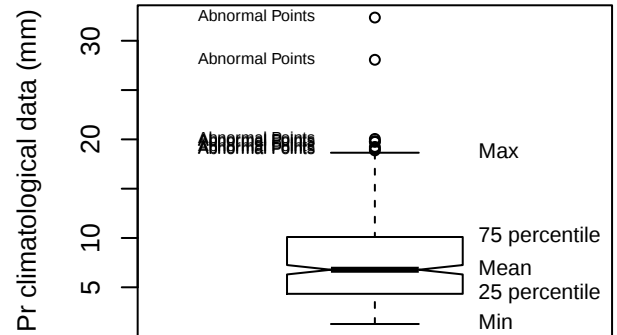
Box plot (STMB)
