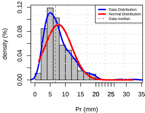
Histogram Distribution (STMB)
